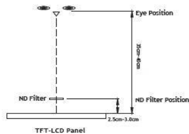
TFT-LCD Panel
